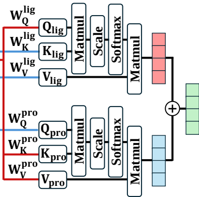
Cross-attention
