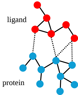
GNN encoder
