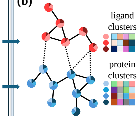
Functionality-based Clustering
