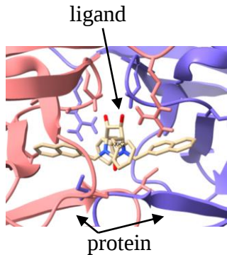
Protein-ligand complex
